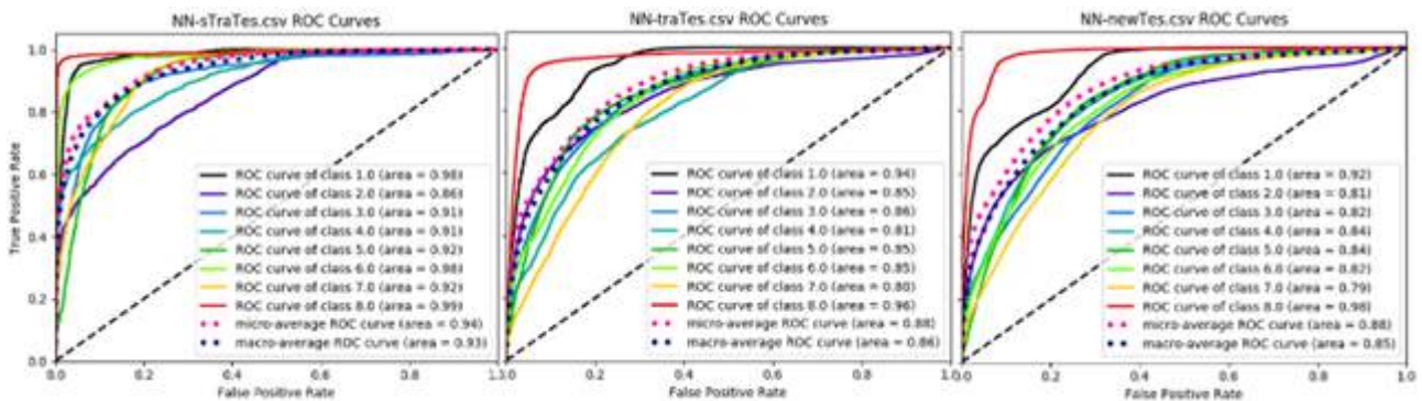
Figure 28: ROC curves for 3 types of testing sets (sTraTes, traTes, newTes)
