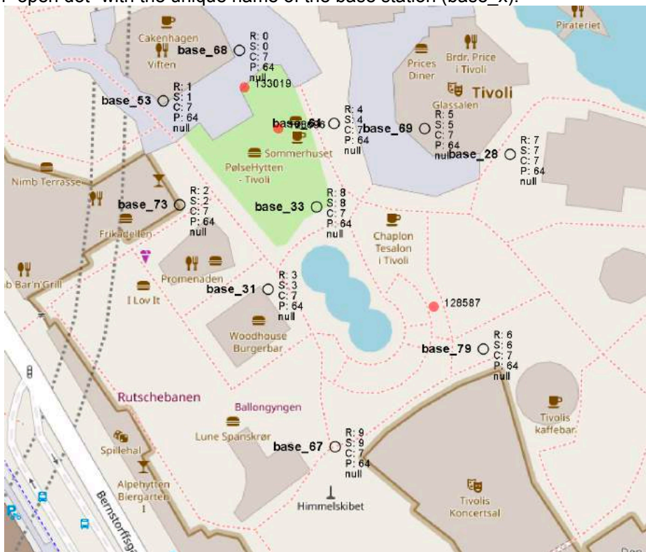
Figure 18: Location of base stations and crowd wristbands
