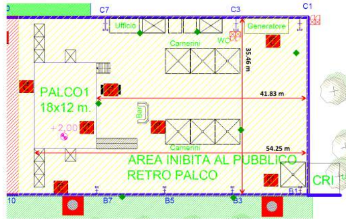
Figure 34: Blueprint, anchor locations and dimensions of the main backstage test area
