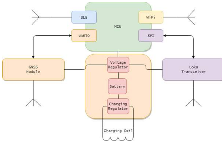
Figure 44: Modular diagram of hardware components in LoTrack tracker
