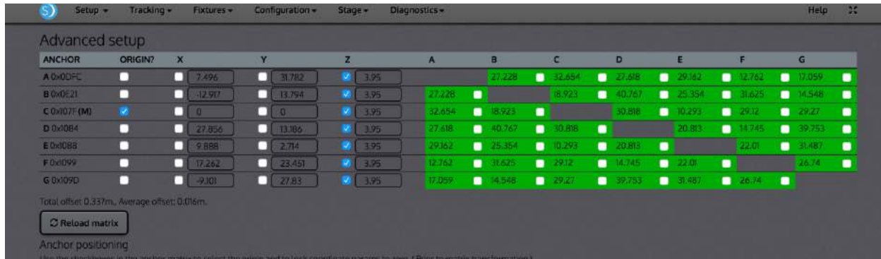
Figure 33: Result of the automatic anchor positioning procedure at KFF2017
