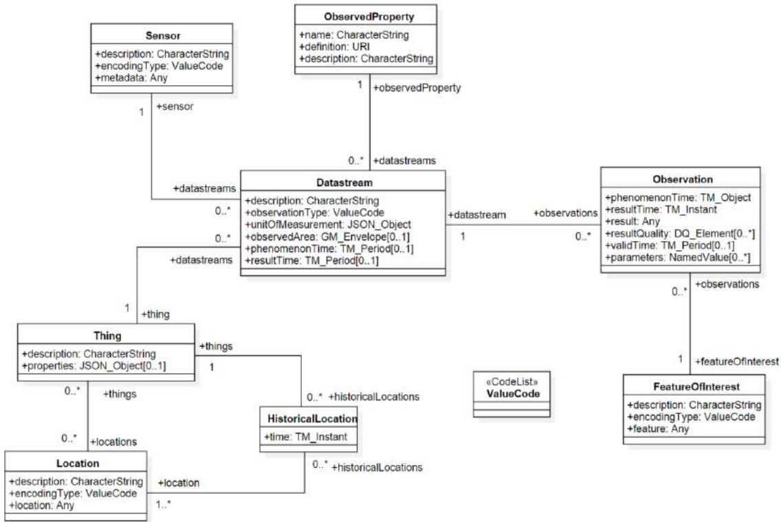
Figure 50: OGC SensorThings Model
