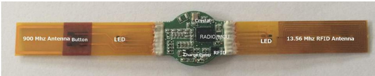
Figure 11: Sendrato smart wristband module 2
