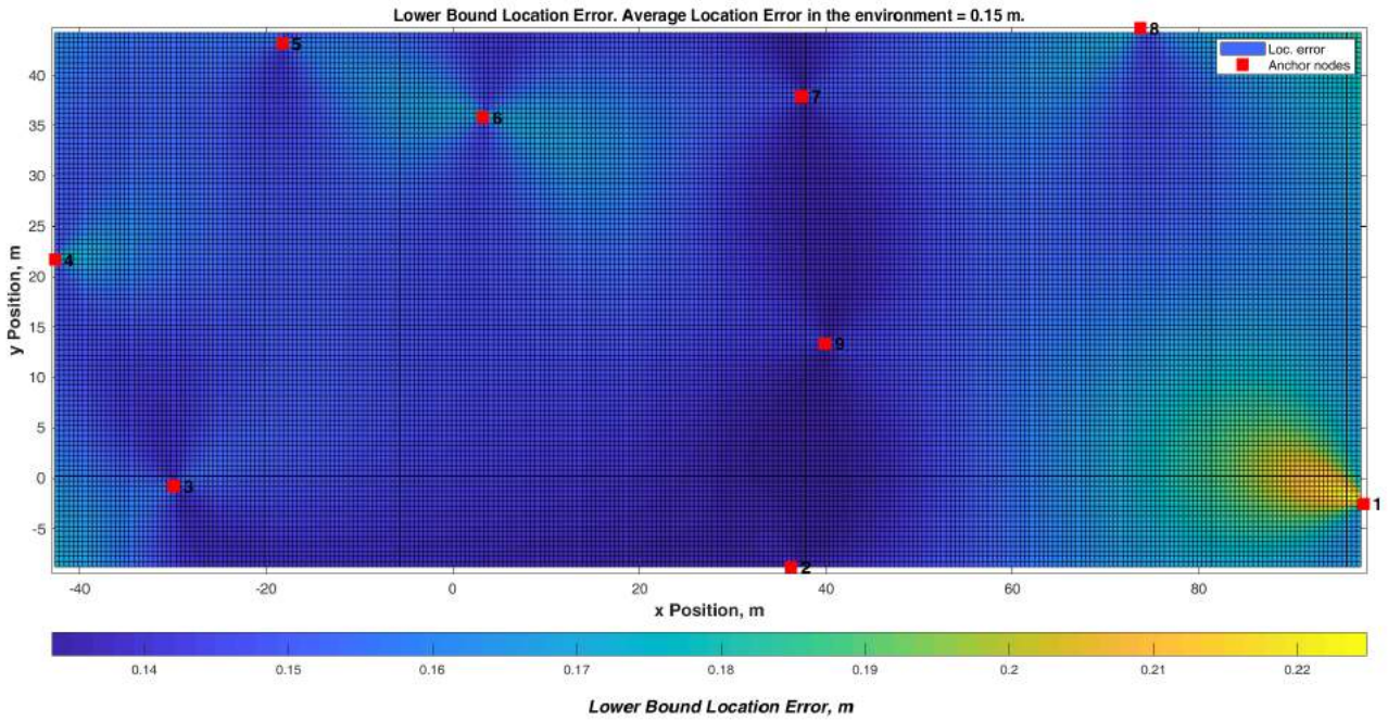
Figure 22: Staff wristbands - CRLB analysis for KFF2018
