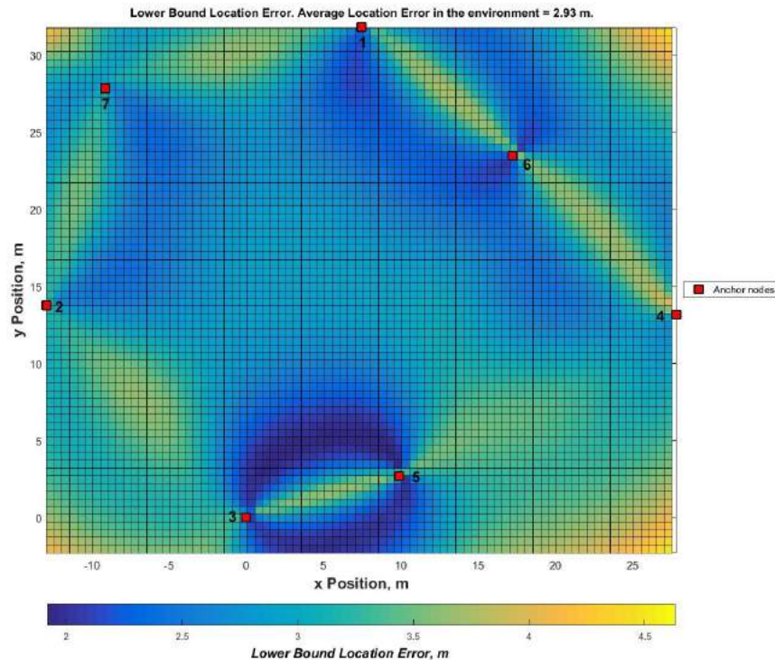
Figure 14: RSSI measurements CRLB analysis
