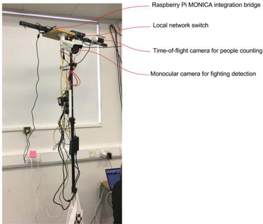
Figure 58: Demonstration of Time-of-flight camera for real-time tracking and counting with MONICA bridge running on a Raspberry Pi on the local network
