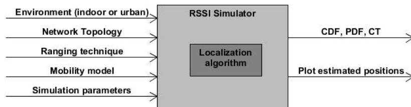
Figure 16: RSSI-based simulator
