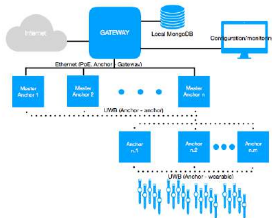
Figure 20: Staff wristbands infrastructure deployment
