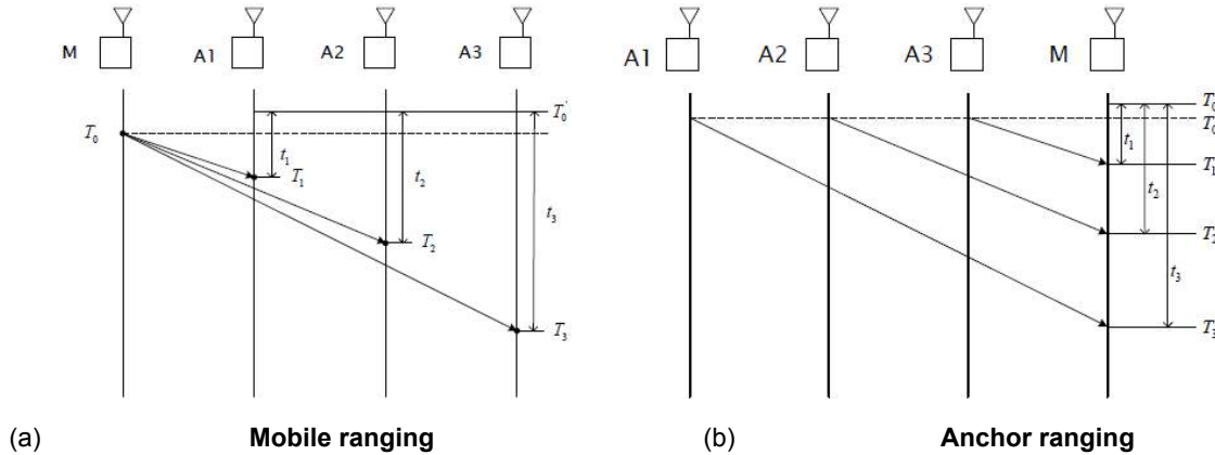
Figure 3: Time-difference-of-arrival ranging
