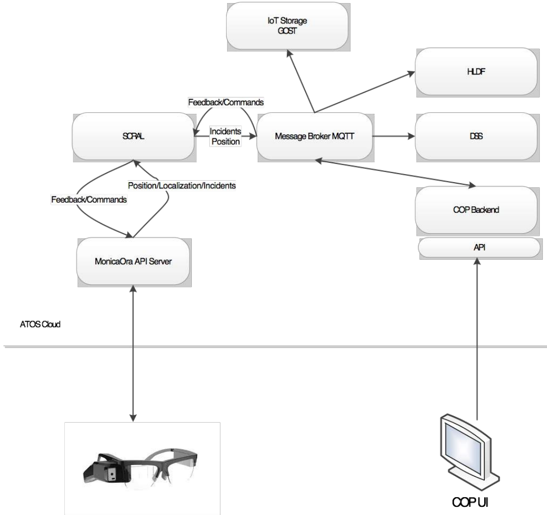
Figure 42: Smart glasses integration
