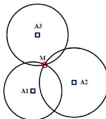
Figure 5: Lateration of three anchors based on RSSI and ToA
