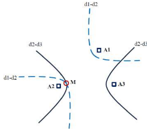
Figure 6: Lateralization of three anchors based on TDoA
