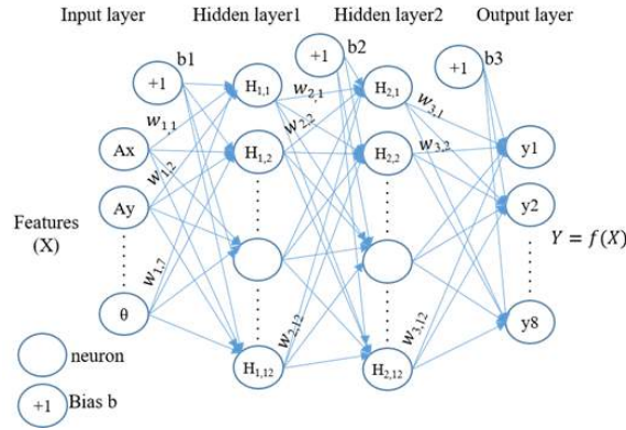
Figure 24: Two hidden layers MLP used in this study
