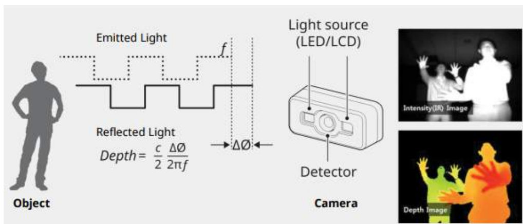
Figure 53: Phase shift of reflected light used to calculate the distance of objects from the sensor
