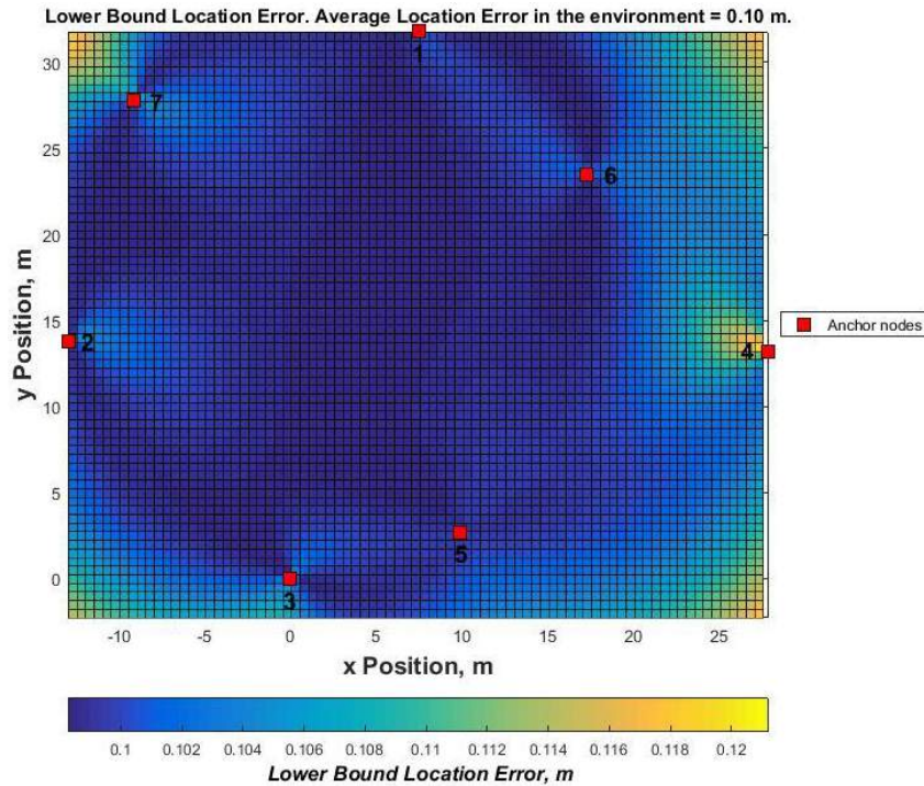
Figure 21: Staff wristbands - CRLB analysis for KFF2017
