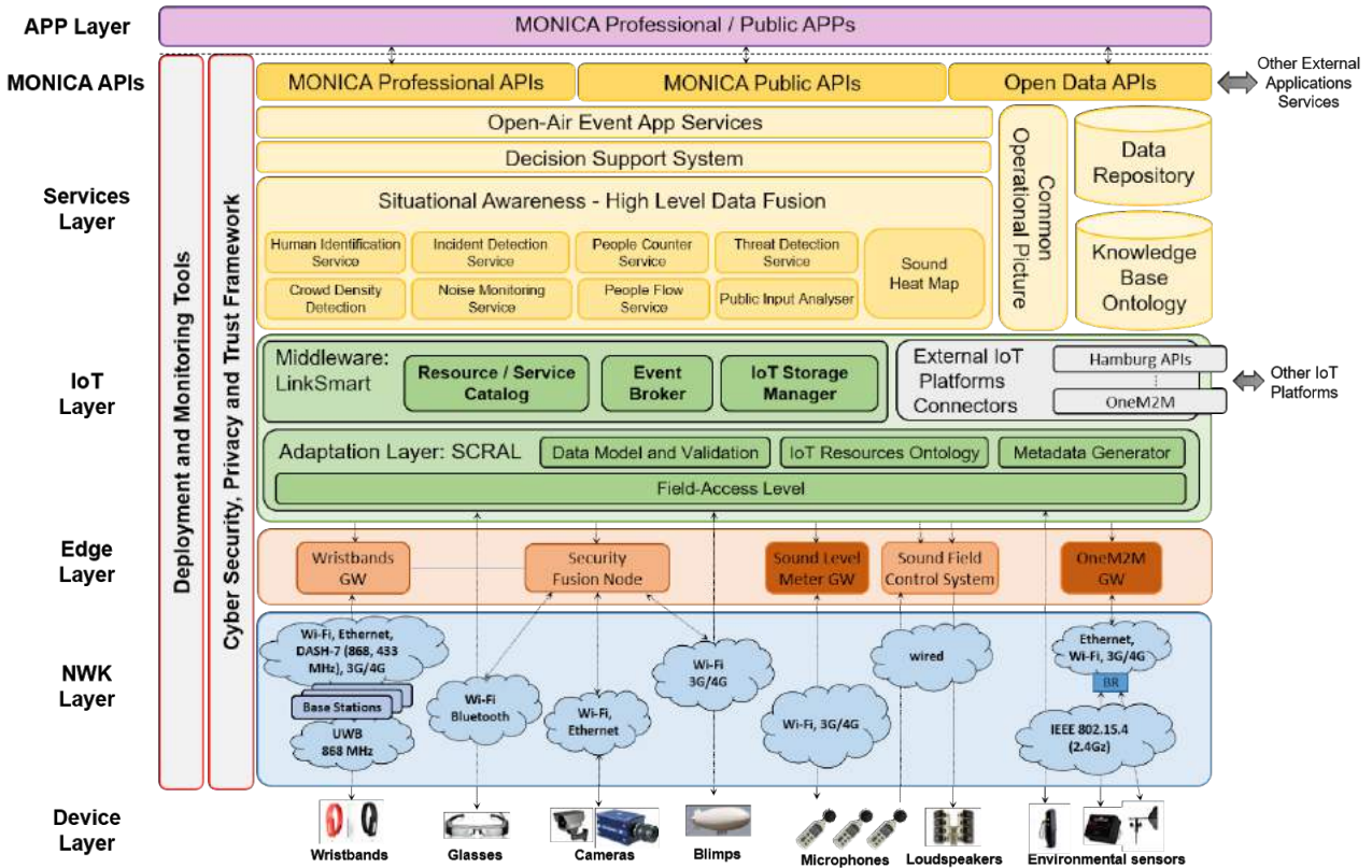
Figure 49: MONICA Architecture
