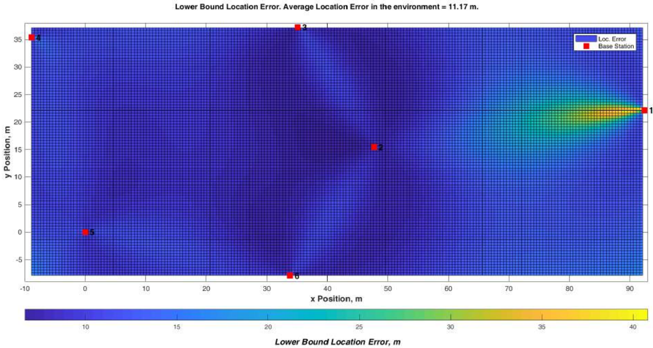
Figure 15: Crowd wristbands - CRLB analysis for KFF2018
