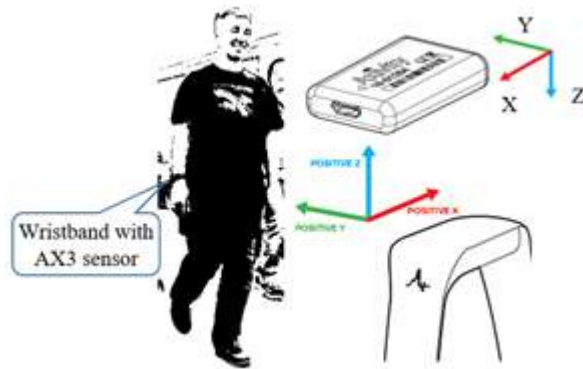
Figure 23: System configuration
